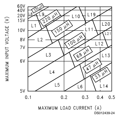
FIGURE 4. LM2594/LM2594HV-3.3
