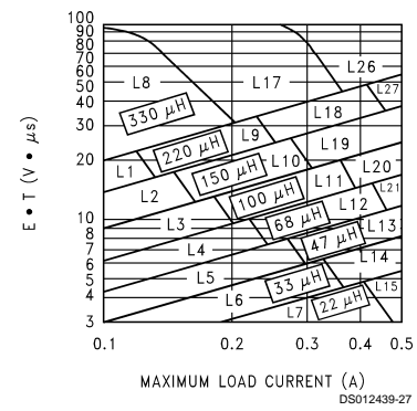
FIGURE 7. LM2594/LM2594HV-ADJ
