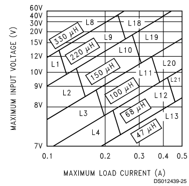
FIGURE 5. LM2594/LM2594HV-5.0
