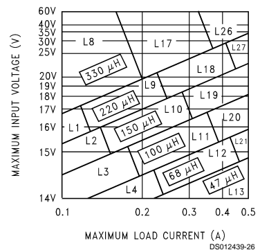
FIGURE 6. LM2594/LM2594HV-12
