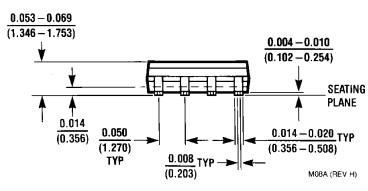
8-Lead (0.150" Wide) Molded Small Outline Package, Order Number LM2594M-3.3, LM2594M-5.0, LM2594M-12 or LM2594M-ADJ JEDEC NS Package Number M08A
